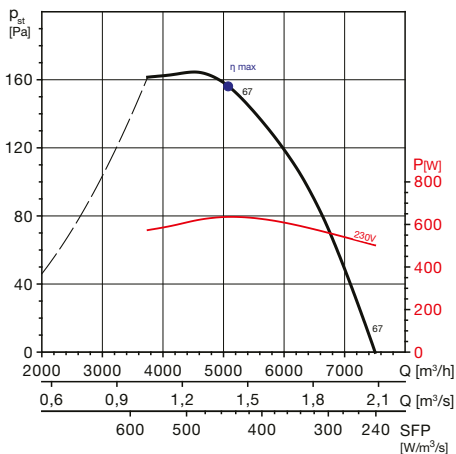
TCBB/4-500 H
