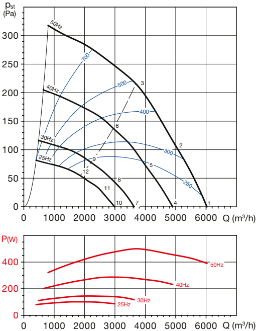
CRHT/6-500 N
