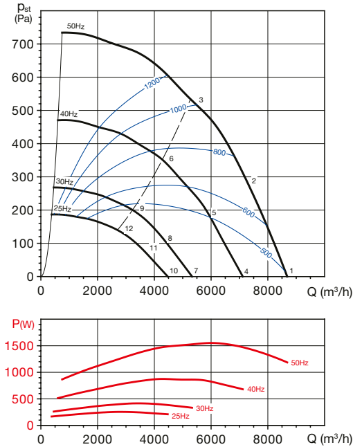
CRHT/4-500 N
