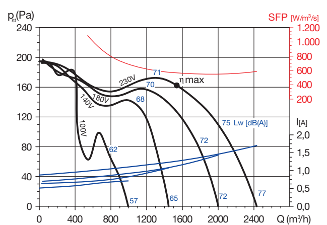
CBM-9/7 245 6P RE VR
