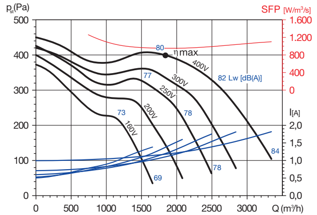
CBM-9/7 550 4PT RE VR
