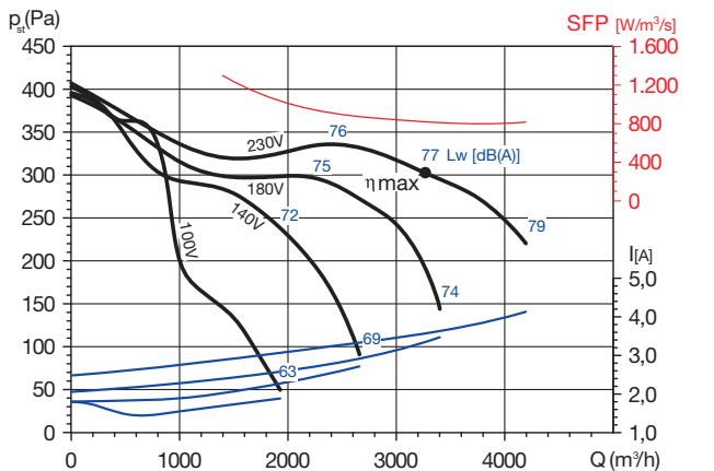
CBM-12/9 515 6P RE VR
