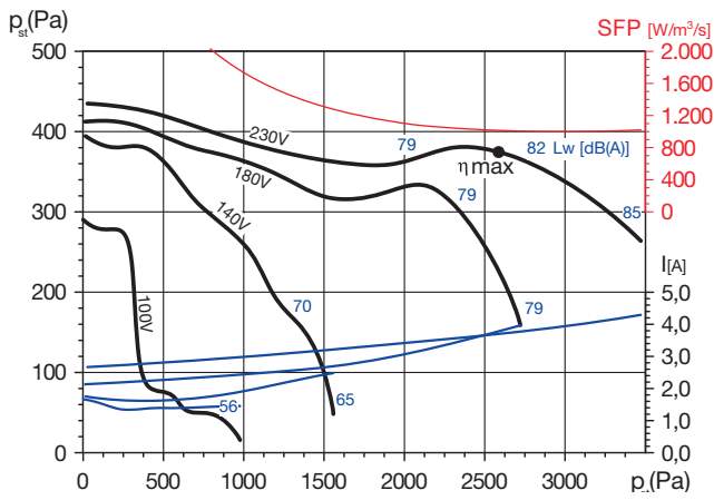
CBM-9/9 550 4P RE VR
