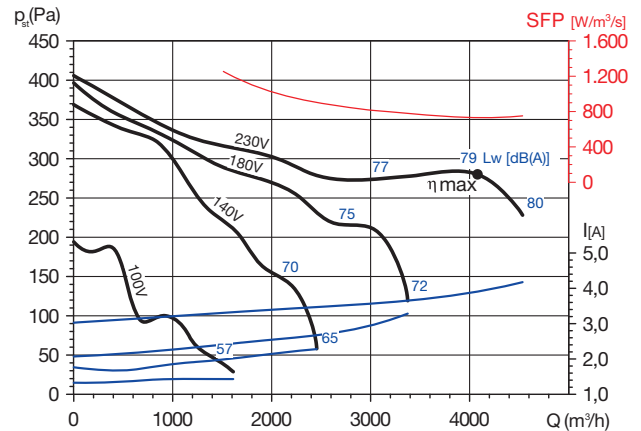
CBM-12/12 515 6P RE VR
