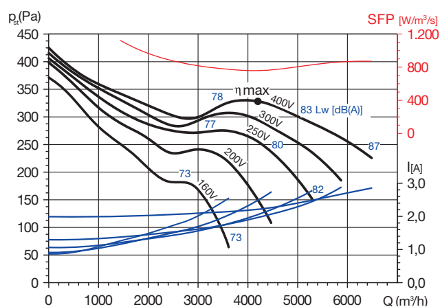
CBM-12/12 550 6PT RE VR
