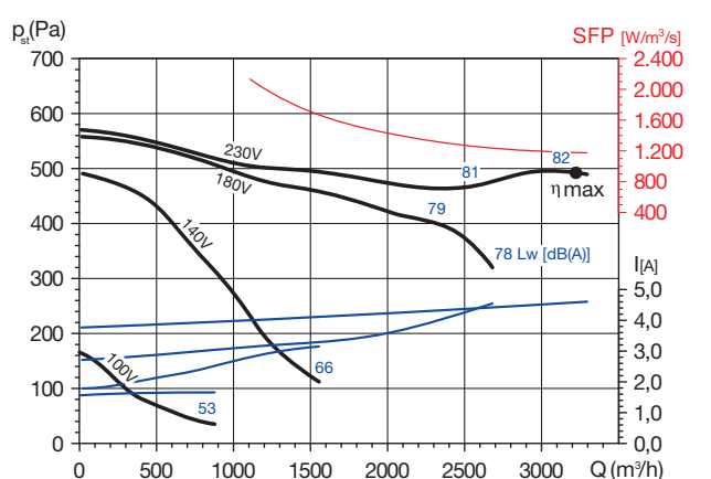
CBM-10/10 600 4P RE VR
