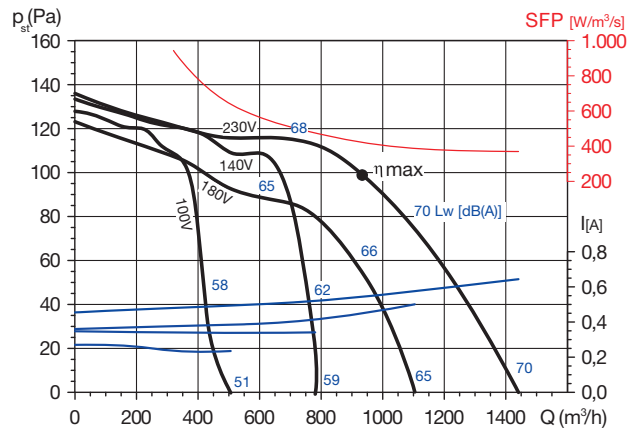
CBM-7/7 72 6P RE VR
