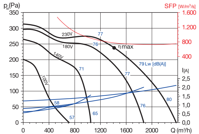
CBM-7/7 300 4P RE VR
