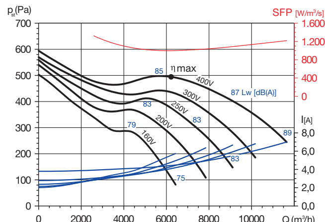
CBM-15/15 2200 6PT RE VR
