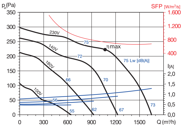
CBM-7/7 147 4P RE VR
