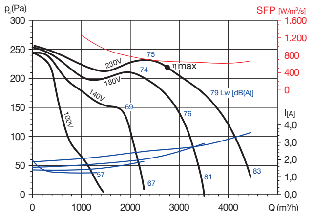
CBM-10/10 515 6P RE VR
