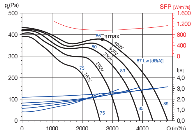
CBM-9/9 550 4PT RE VR
