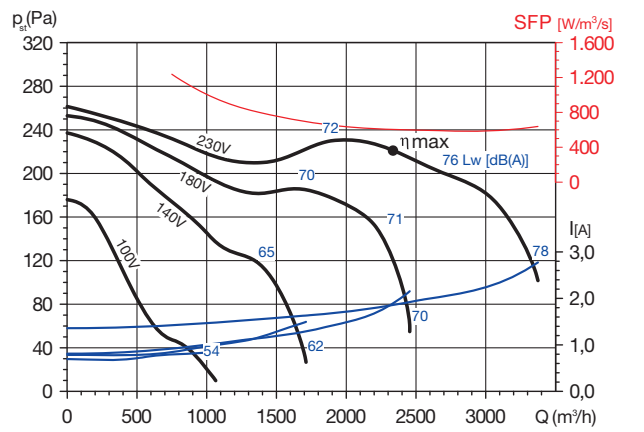
CBM-10/10 245 6P RE VR
