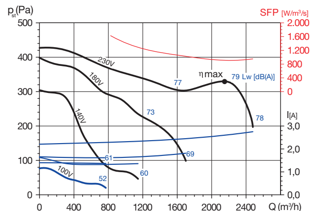
CBM-9/9 300 4P RE VR
