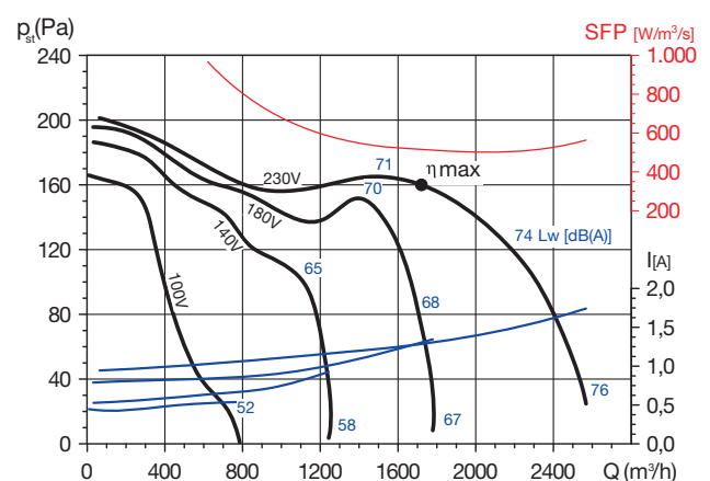
CBM-9/9 200 6P RE VR
