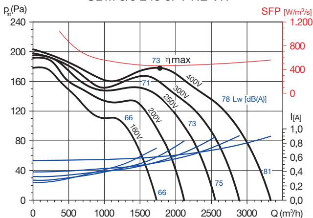
CBM-9/9 245 6PT RE VR
