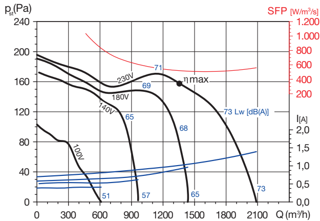
CBM-9/7 200 6P RE VR
