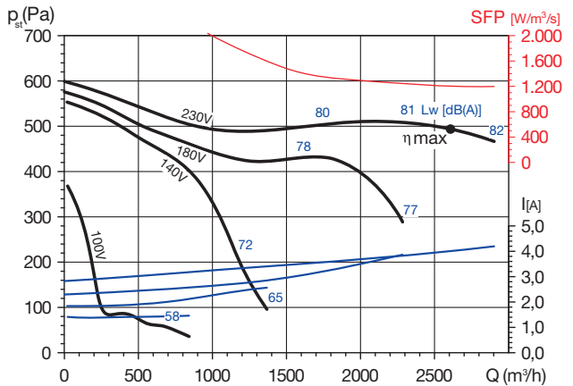
CBM-10/8 550 4P RE VR
