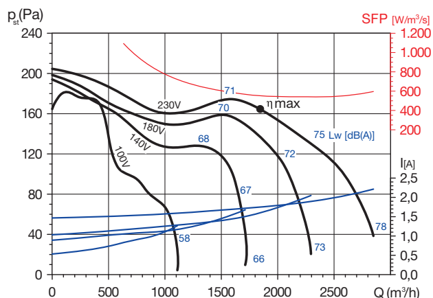
CBM-9/9 245 6P RE VR
