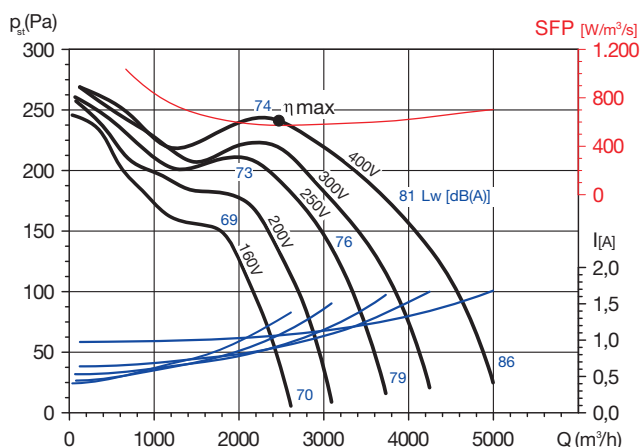
CBM-10/10 350 6PT RE VR
