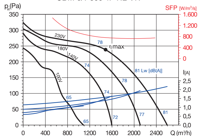
CBM-9/7 300 4P RE VR
